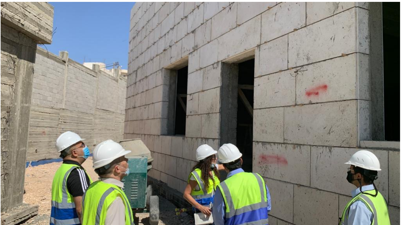
Number of stones are broken, the gaps should be unified and the part of façade needs to be cleaned
